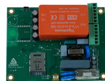
AFF/001-SMS Flash'n'Text™ PCB
