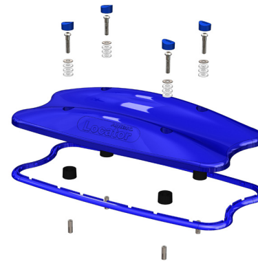
Locator™ with Concrete Fixing Kit Exploded View
