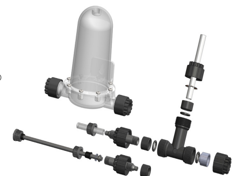
Exploded View of Large Bore Fittings Range
